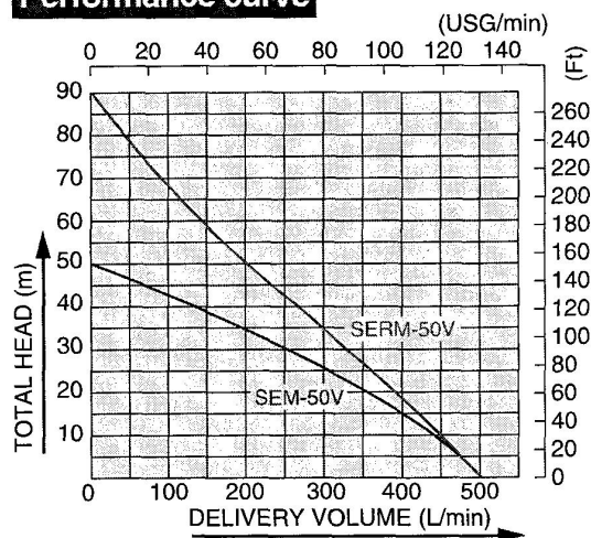
Performance curve
